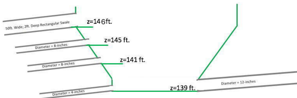
Figure 2: Schematic elevation-view sketch of pond.
